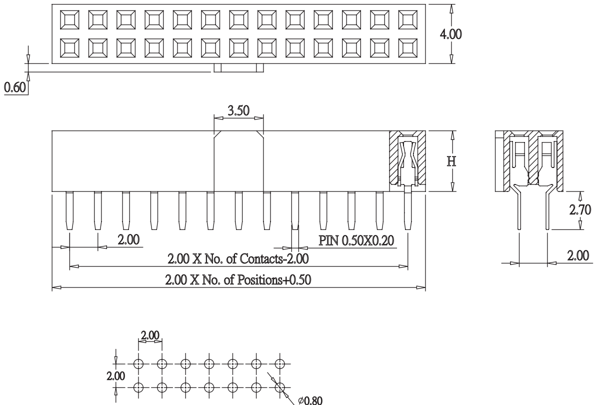
Recommended PCB Layout (PCB TOLERANCE \pm 0.05 )
